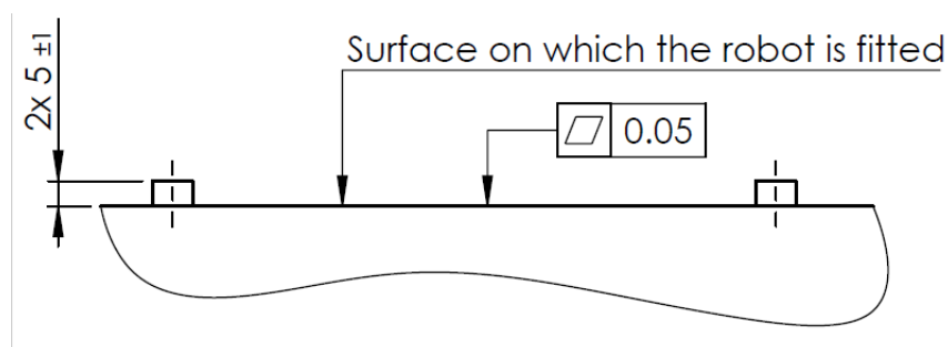
1.2: Monteringsplate for robotbase
